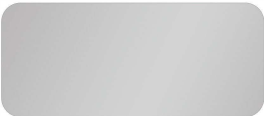
Natural (Uncoated)
