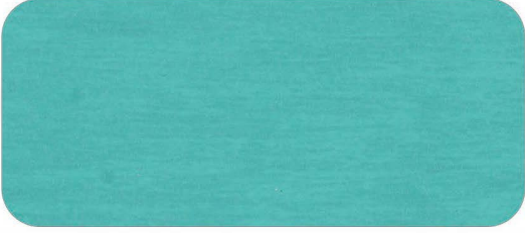
Copper Patina
