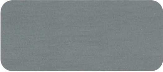
Zinc Patina
